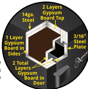
Cutaway drawing showing the TF Series interior construction
