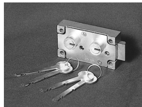
U.L. LISTED DUAL NOSE KEY LOCK Dual control safe deposit lock requires two different keys to open safe.
