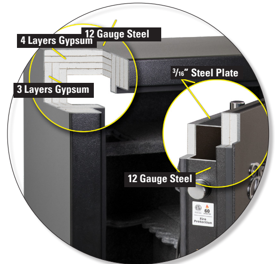
SF6036E5 Standard Interior
