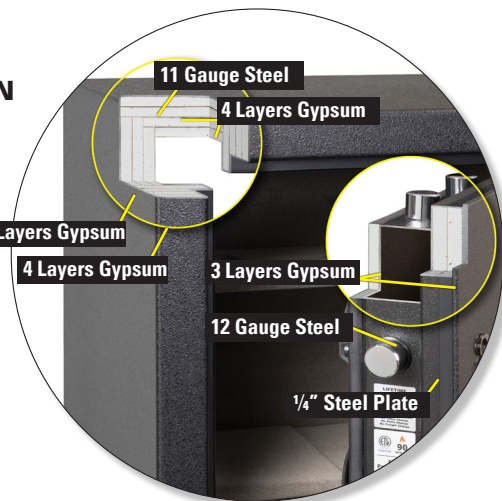
NF6030E5 Standard Interior
